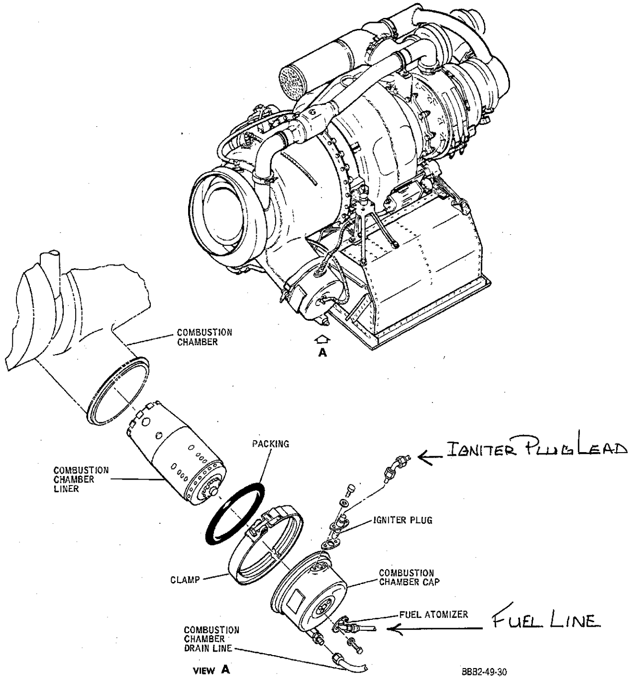
Figure 201. Combustion Chamber Liner -- Installation (Sheet 1) / 49-20-01-990-801 Sheet Effectivity: AAL 601-703
