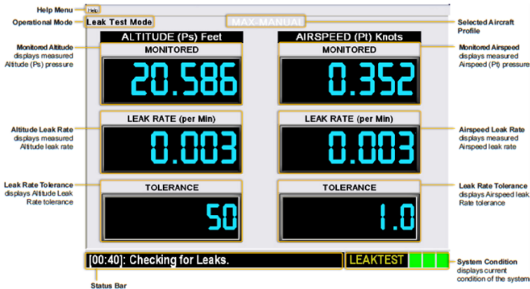
Figure 5: DPS500NG Leak Test Mode
