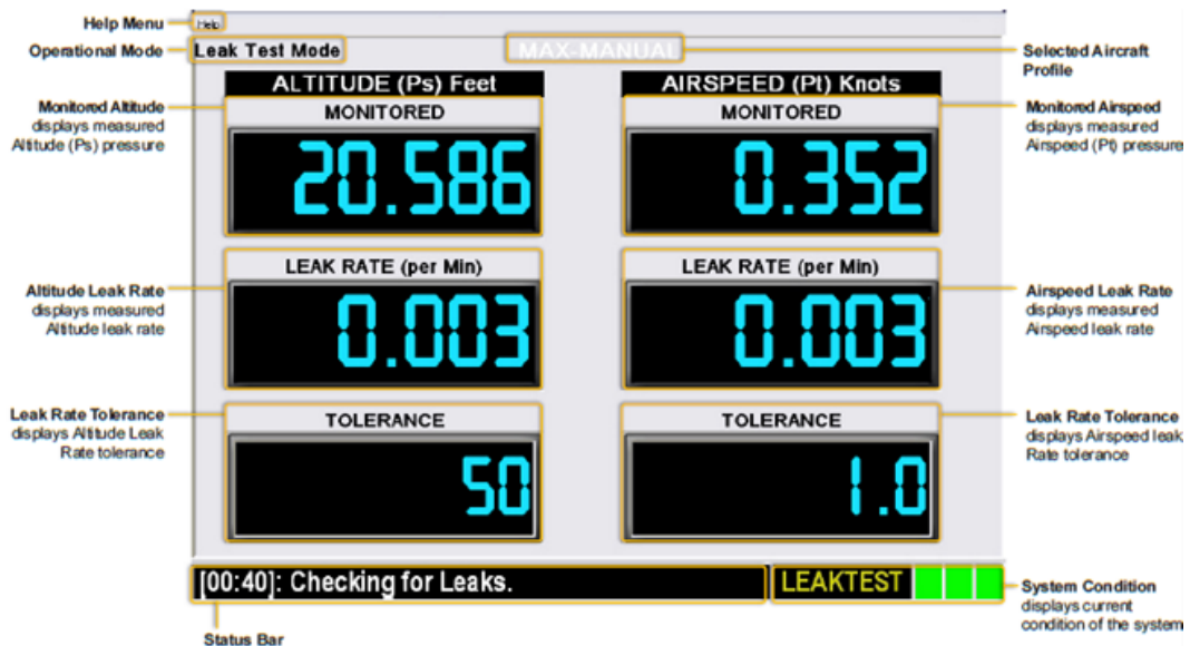
Figure 7: DPS500NG Leak Test Mode
