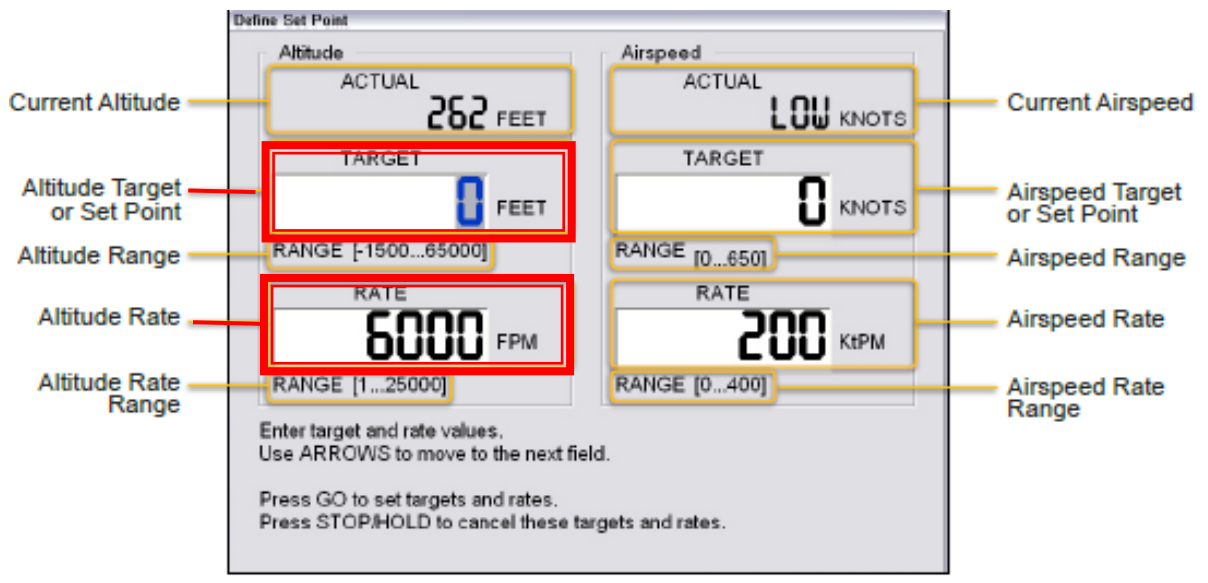
Figure 6: DPS500NG Define Setpoint Window (Altitude)
